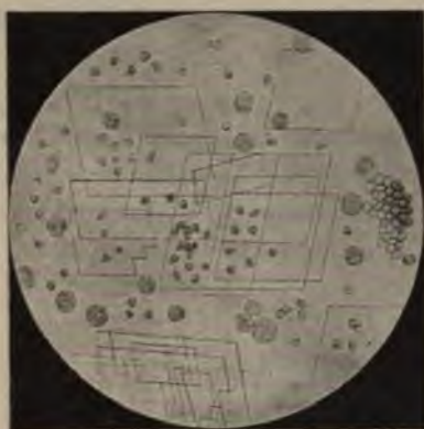
FIG. 52.—Cholesterol. (After Funke.)
